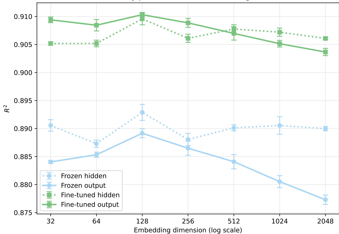
Hand velocity prediction R^2 vs. embedding dimension
