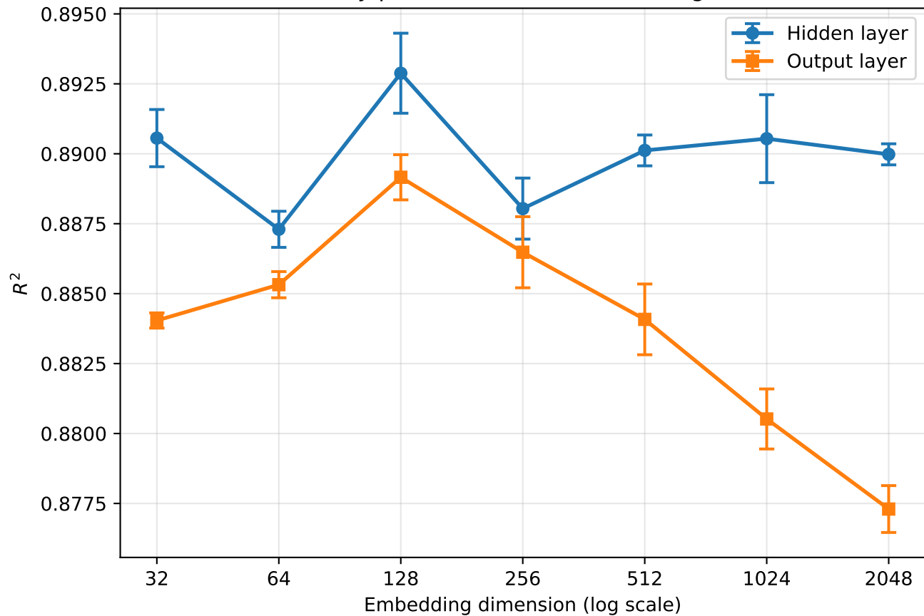
Hand velocity prediction R^2 vs. embedding dimension
