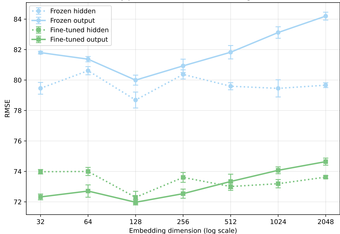
Hand velocity prediction RMSE vs. embedding dimension
