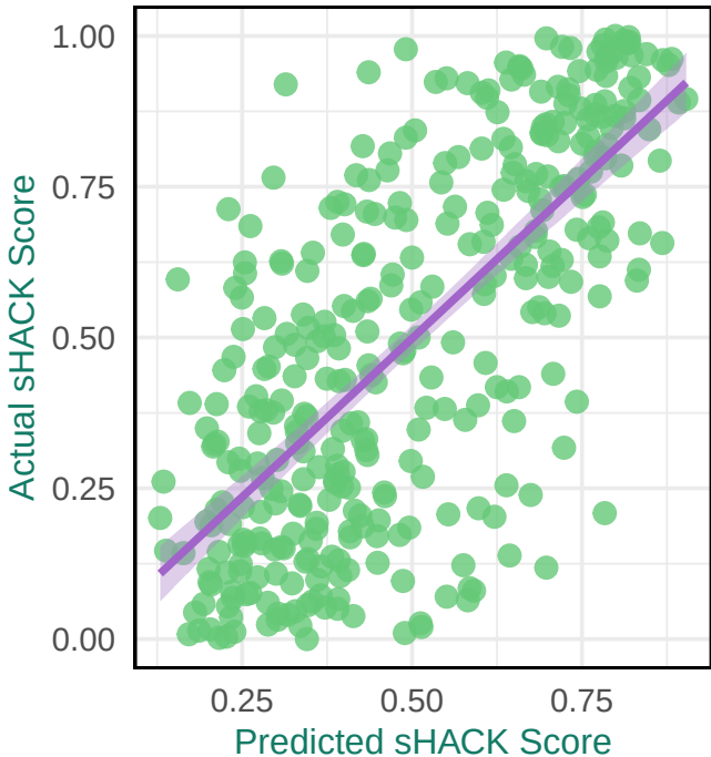
Predicted vs Actual sHACK Score (40Feat
