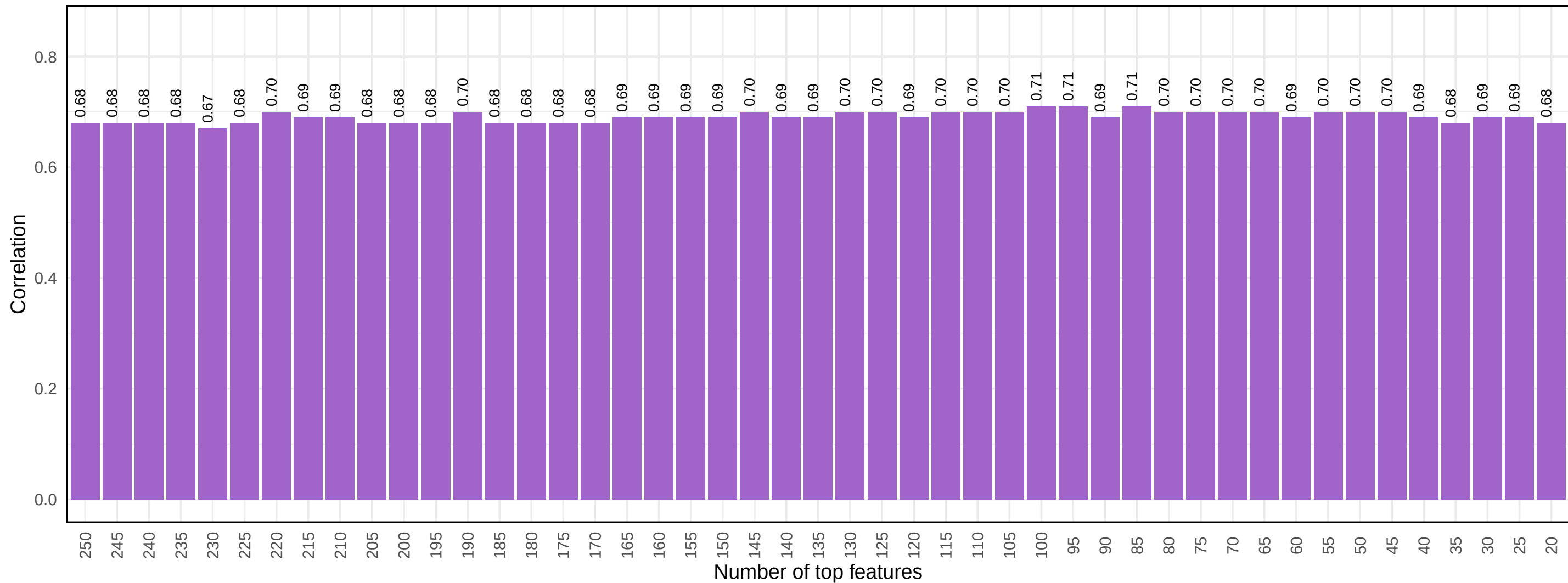
Correlation across different numbers of top features
