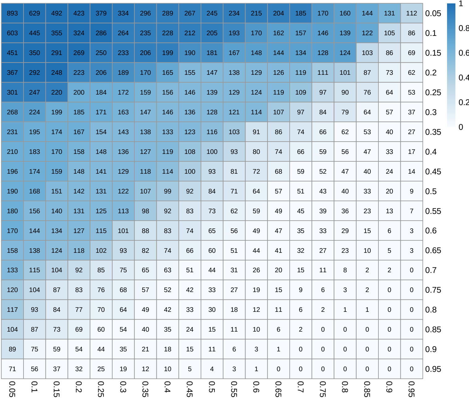
Proportion of microbiomes with ...90% cumulative abundance
