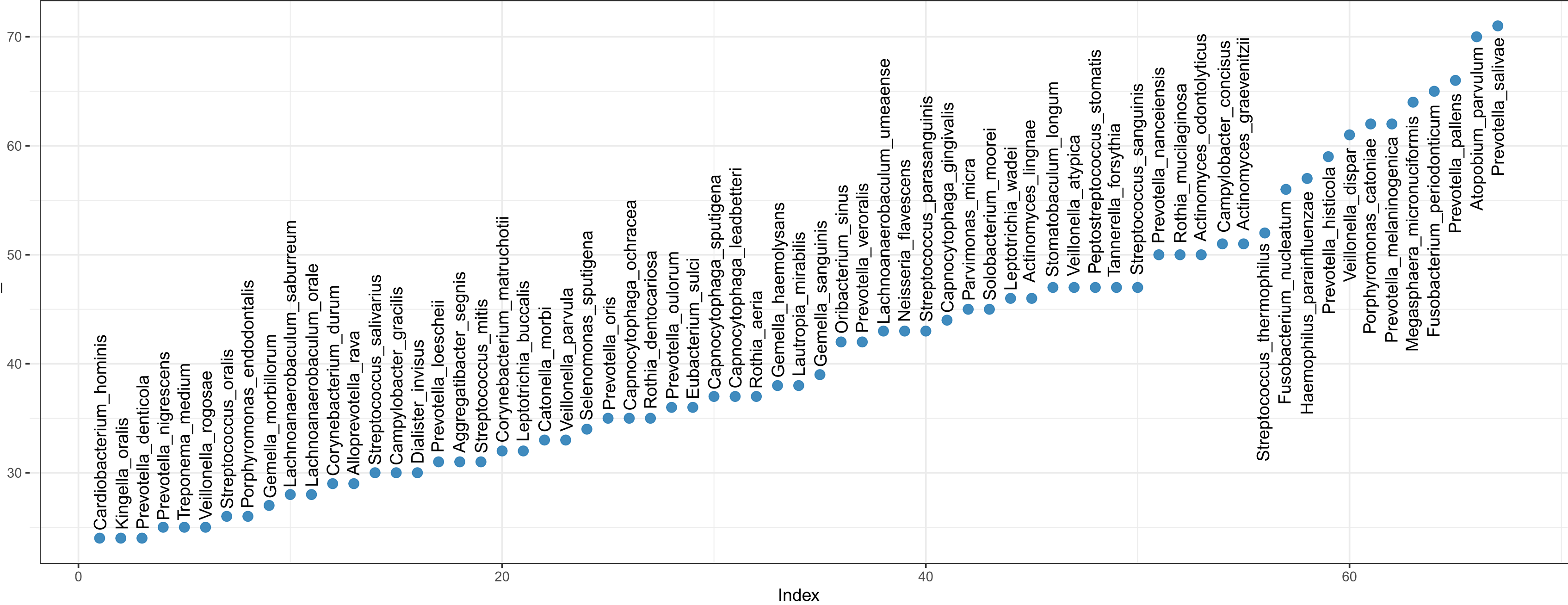
studies_detected
