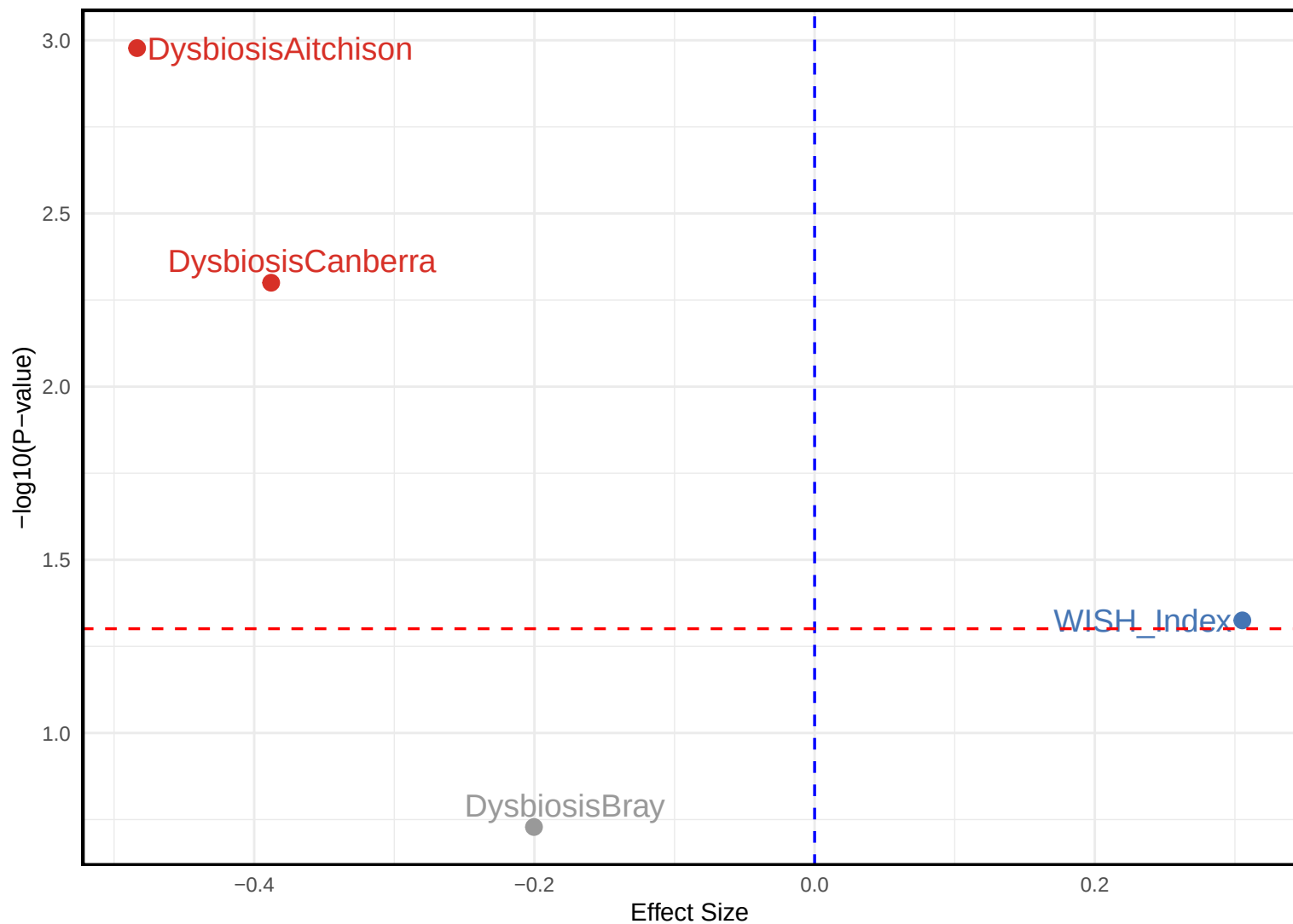
Comparison of Microbiome Indices
