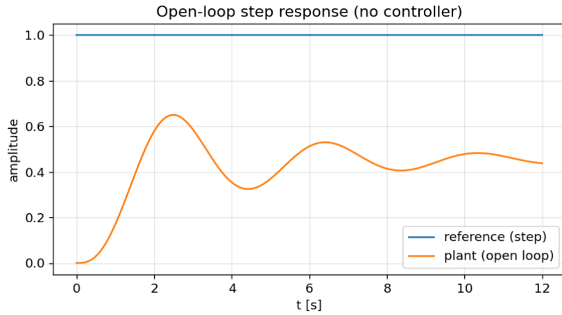
Figure 4: Open-loop step response (no controller): the plant oscillates and does not track the reference.
