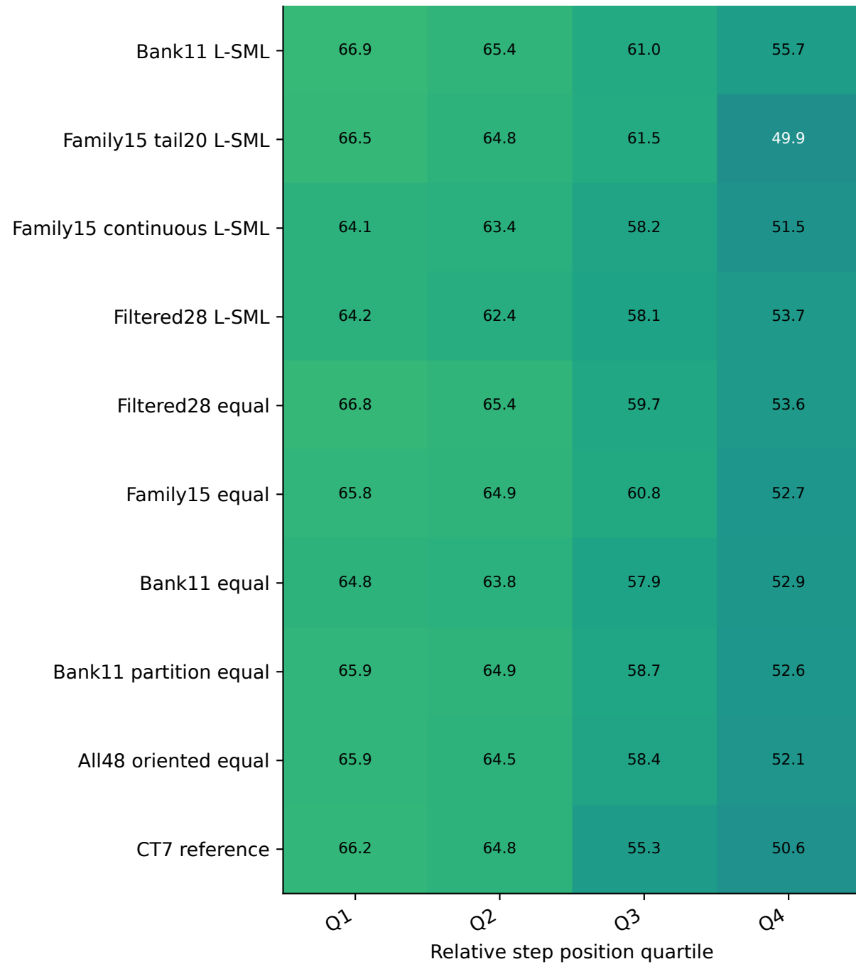
Socratic / QwQ-32B
