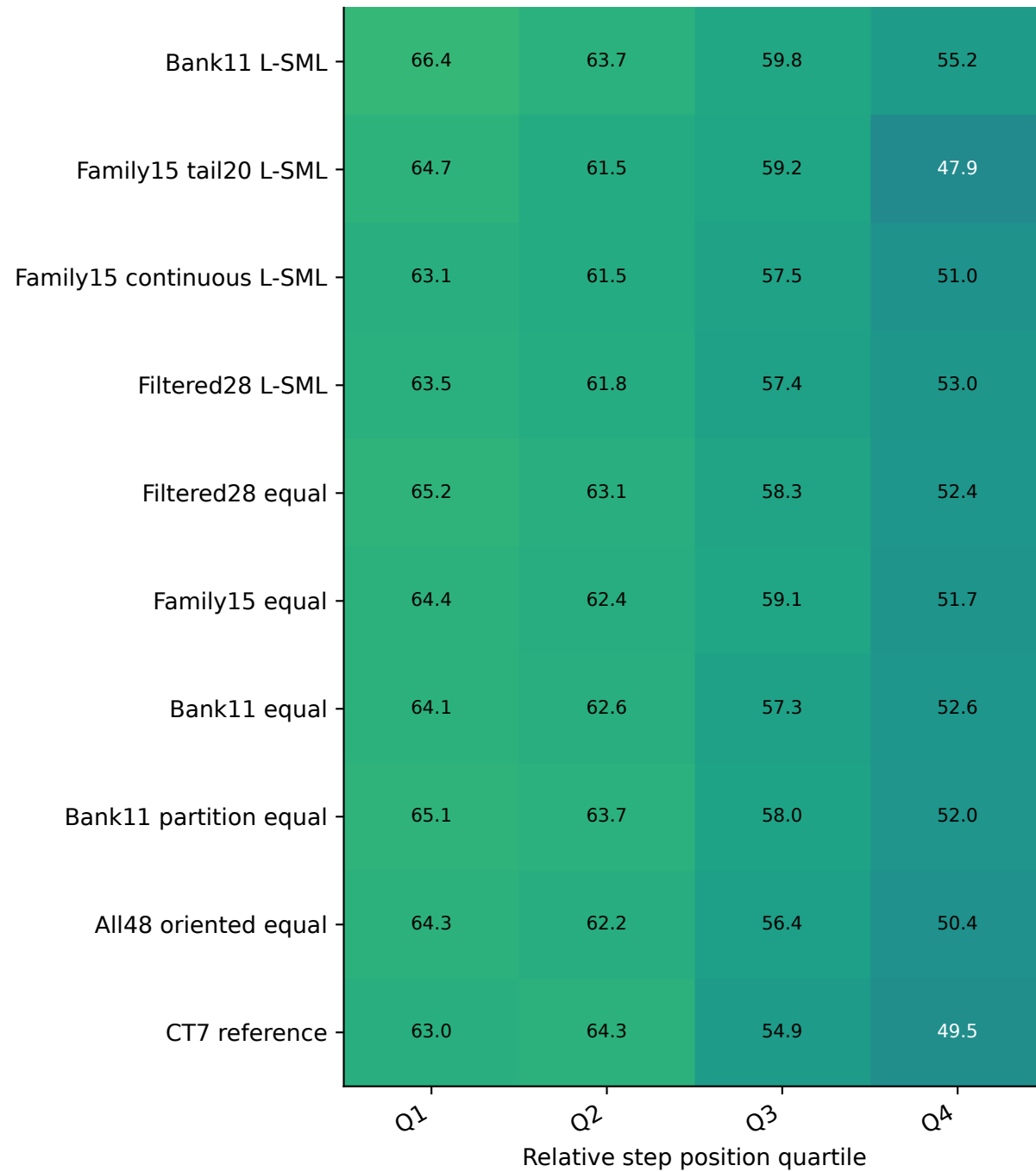
Socratic / Qwen3-8B
