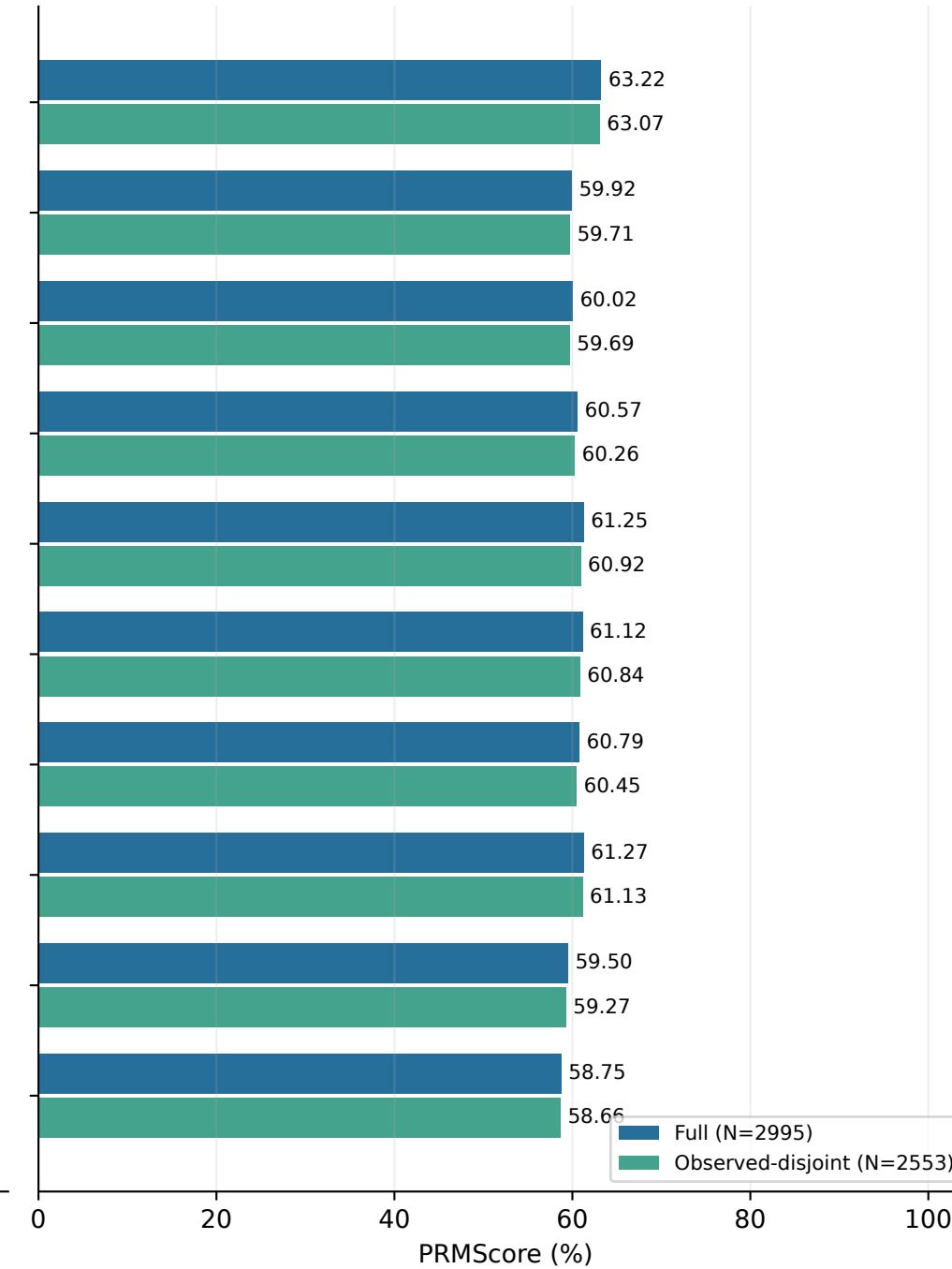
Socratic / Qwen3-8B
