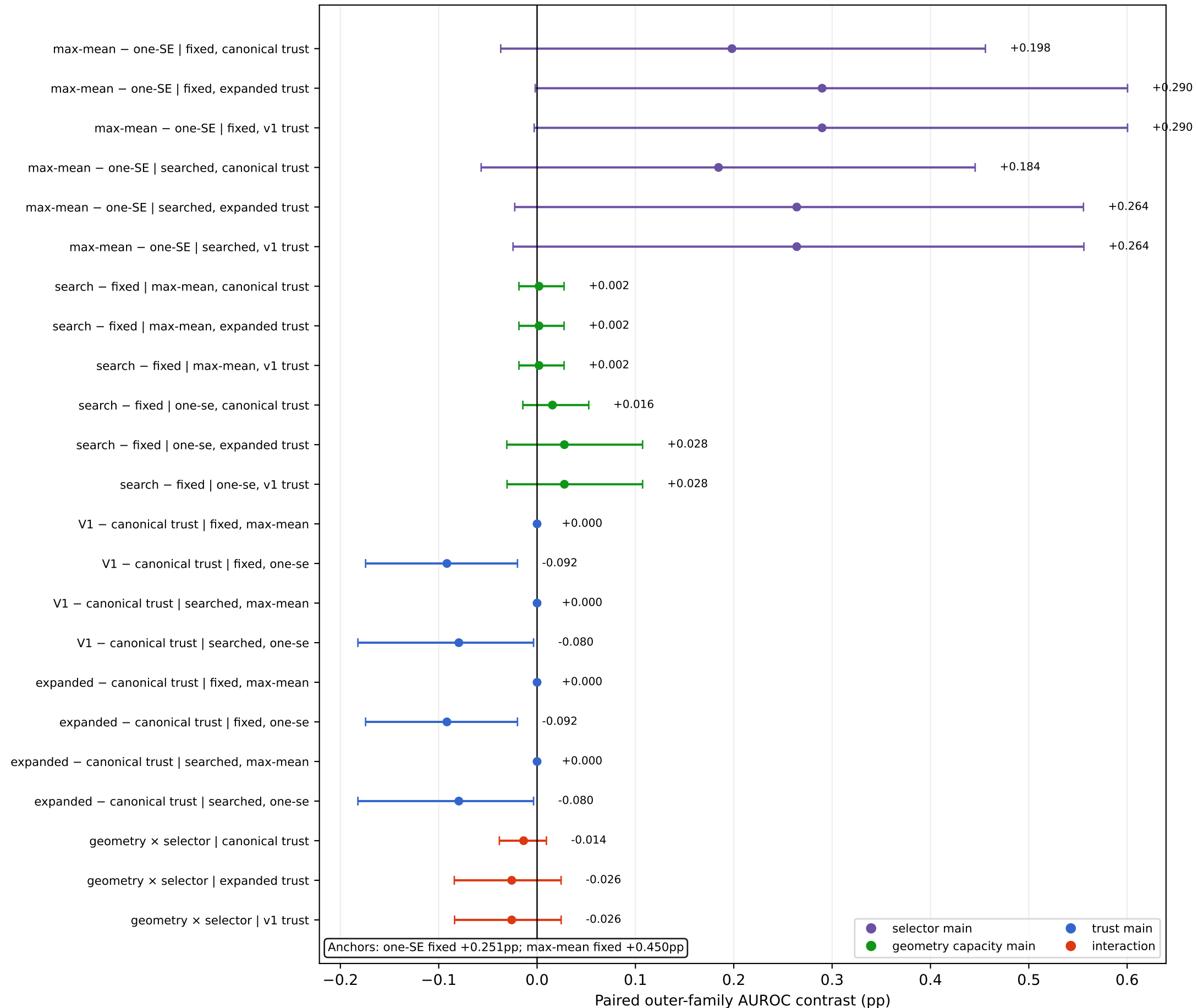
Plot 01 · Controlled factorial forest Selector, geometry-capacity, trust-grid, and interaction contrasts
