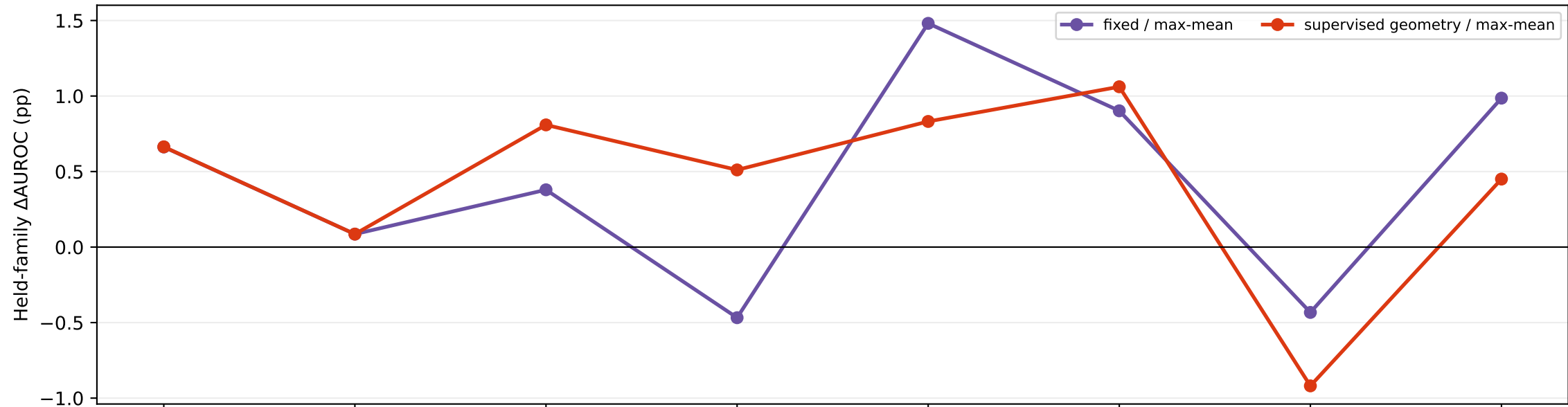
Max-mean policy
