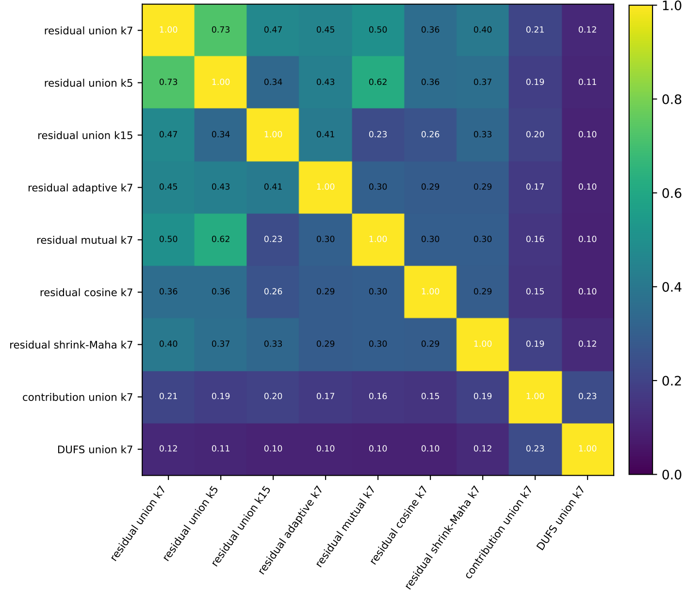
Mean weighted-edge Jaccard
