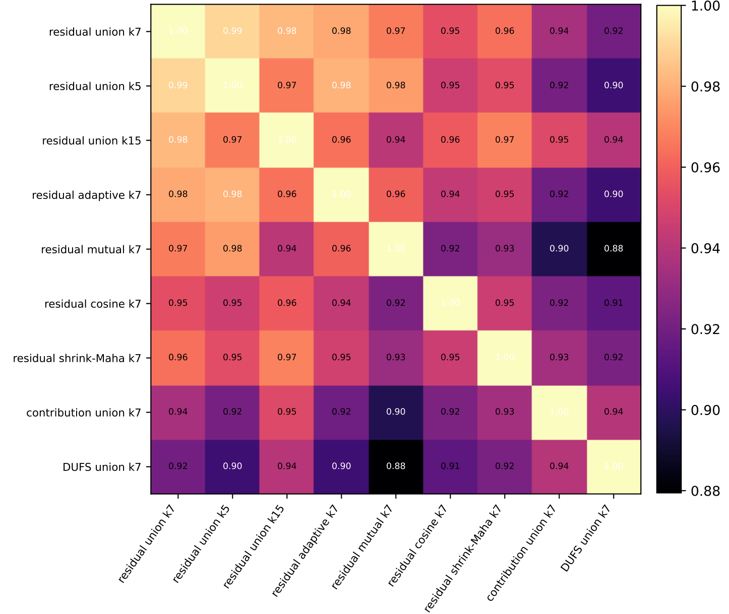
Mean trace-normalized operator cosine
