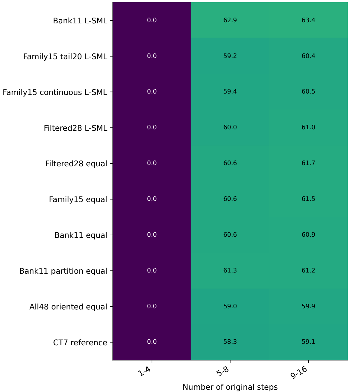
Socratic / Qwen3-8B
