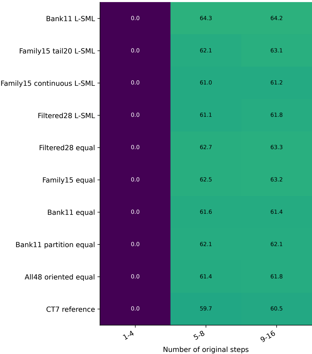
Socratic / QwQ-32B
