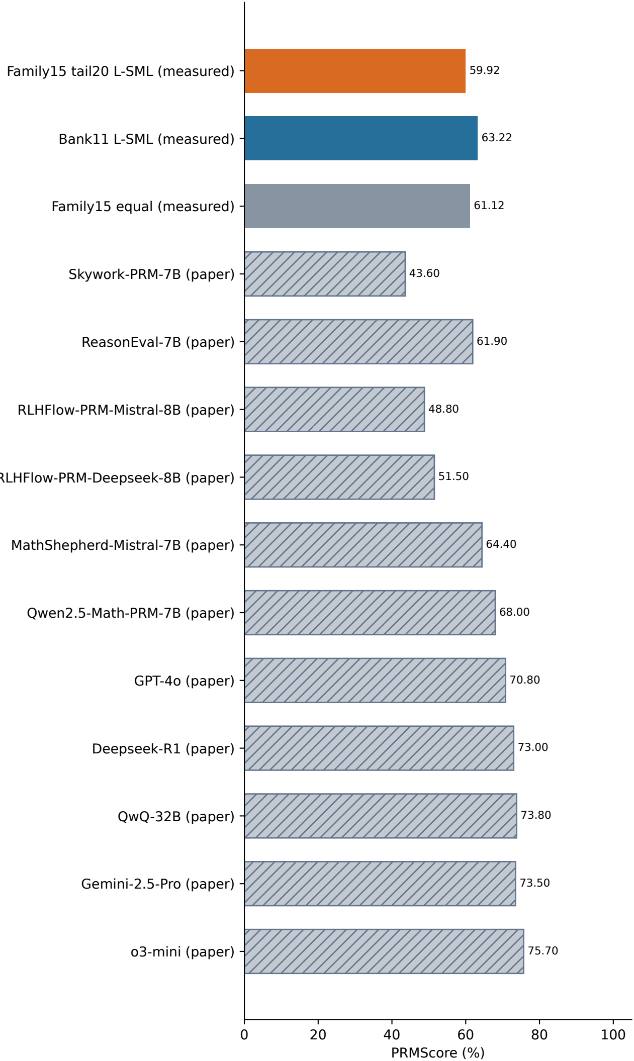
Socratic / Qwen3-8B
