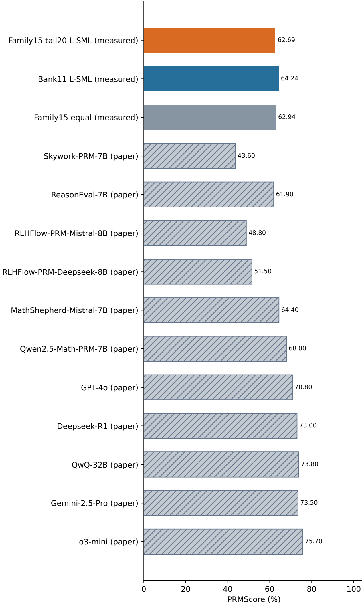
Socratic / QwQ-32B
