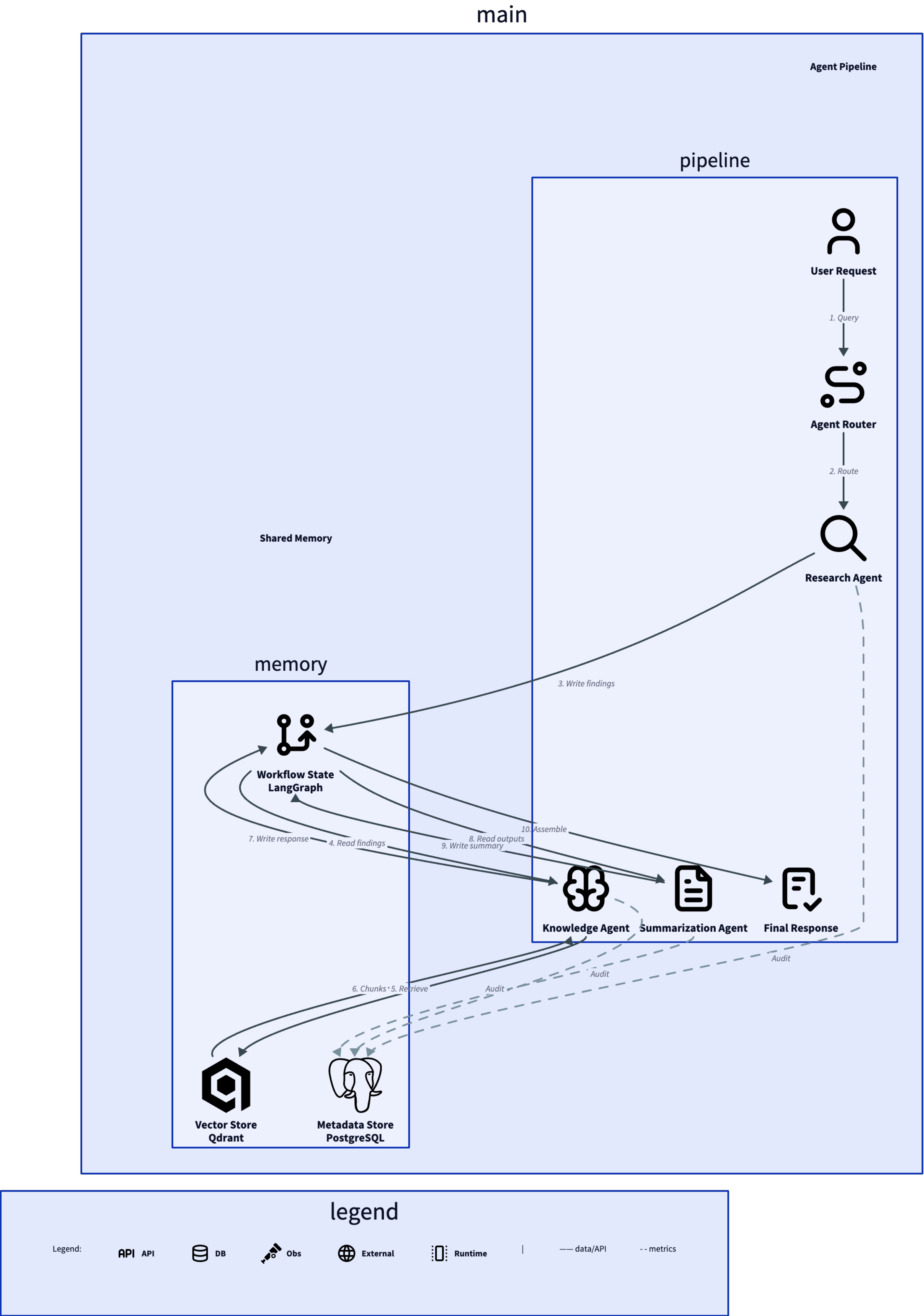
Agent Interaction Flow
