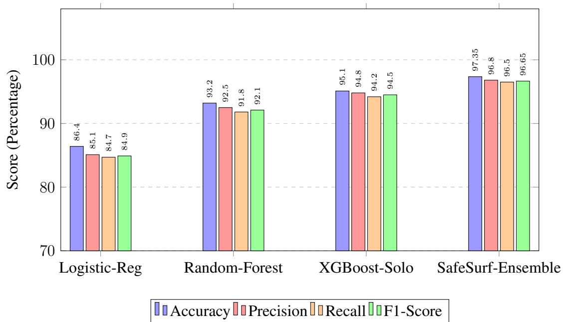
Figure 7.6: Performance Comparison Against Baseline Models (Multi-Metric Analysis)
