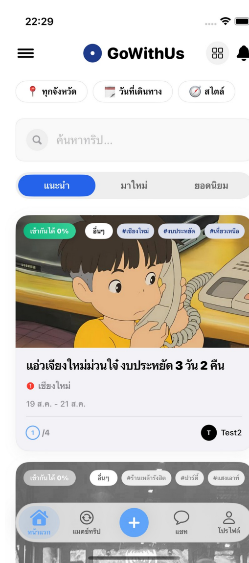
: HomeView
