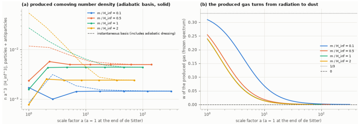
Figure 19: EXP-4 (a) the produced comoving number density na^3 (adiabatic basis solid, instantaneous basis dashed), and (b) the equation of state of the produced gas with its frozen spectrum, from nearly 1/3 at a = 1 to dust.
