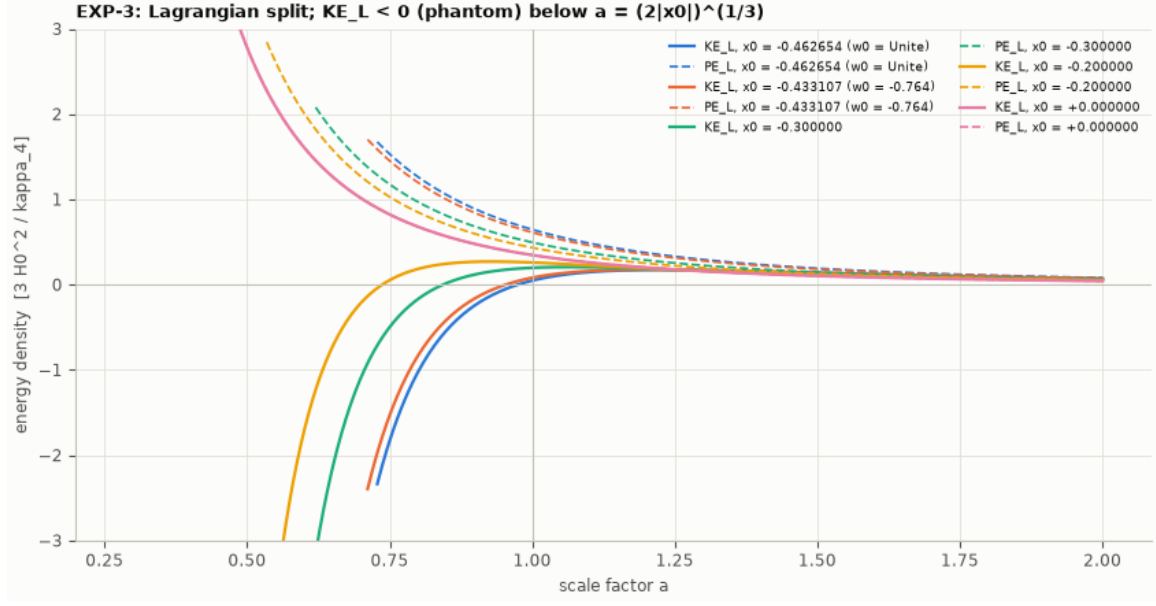
Figure 11: EXP-3 Lagrangian split: KE_L (solid) turns negative, and w drops below -1 , for a < (2|x_0|)^{1/3} ; PE_L (dashed) stays positive.
