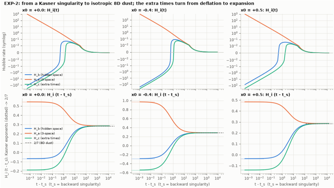
Figure 5: EXP-2 Hubble rates of the hidden space, 3-space and the extra times against t - t_s (top, symmetric log scale), and H_i(t - t_s) with the Kasner exponents dotted and the 8D dust value 2/7 dashed (bottom), for the three runs.
