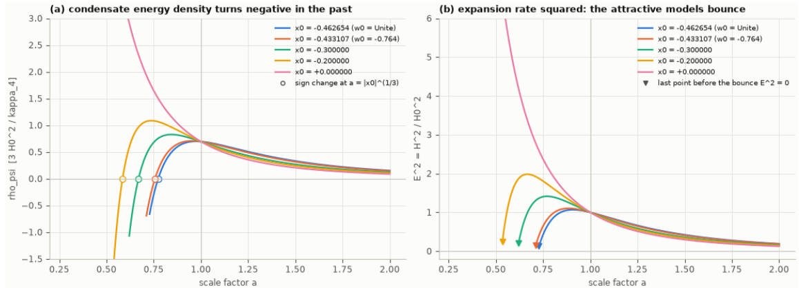
Figure 10: EXP-3 (a) the condensate energy density \rho_\psi(a) , which changes sign at a = |x_0|^{1/3} (circles), and (b) E^2 = H^2/H_0^2 , which reaches zero at the bounce for every attractive model (triangles: last point before the bounce).
