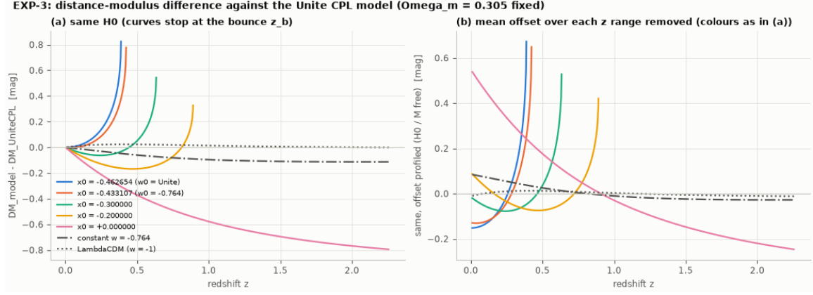
Figure 12: EXP-3 distance modulus minus that of the Unite CPL model ( \Omega_m = 0.305 fixed) for the five couplings, a constant w = -0.764 and \Lambda CDM: (a) same H_0 , curves ending at the bounce; (b) with the mean offset over each curve's redshift range removed ( H_0 and absolute magnitude free).
