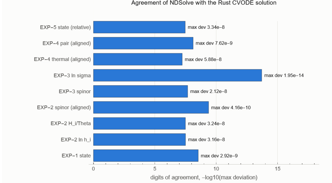
Figure 25: Agreement of NDSolve with the Rust CVODE solutions, as digits of agreement -\log_{10} of the maximum deviation, for each experiment.
