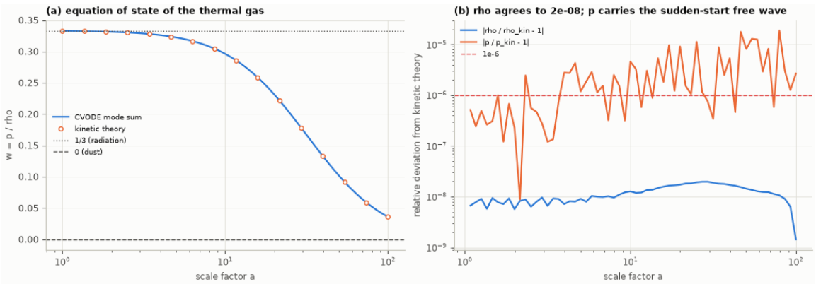
Figure 2: EXP-4: the thermal gas goes from w = 1/3 (radiation) towards w = 0 (dust) as the universe expands; the CVMODE mode sum agrees with kinetic theory
