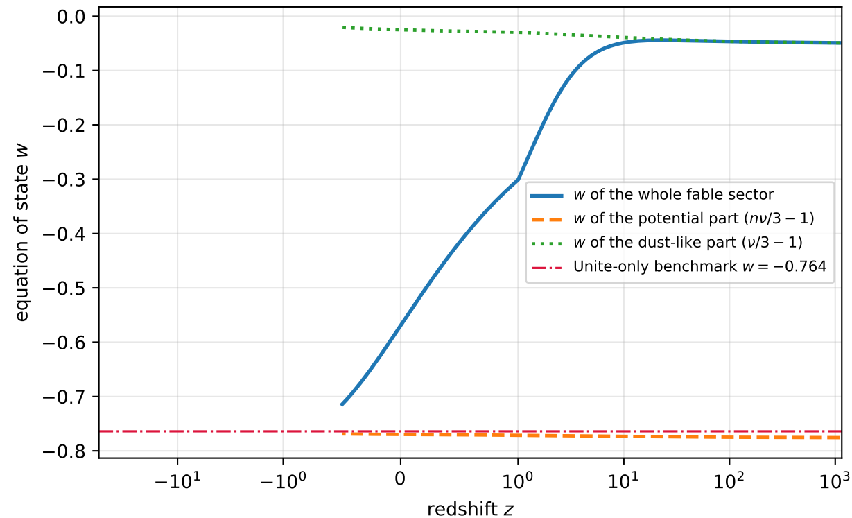
fableSpinor equation of state ( n = 0.236 , \xi = 0.15 )
