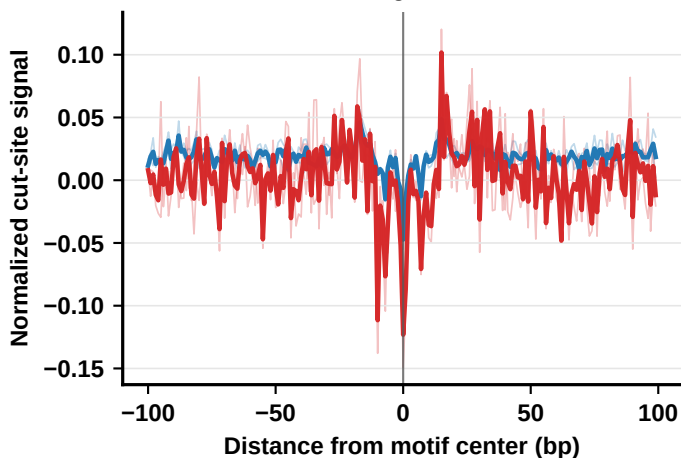
TCF7 (MA0769.3) T-cell-associated regulator, n=9,603 sites
