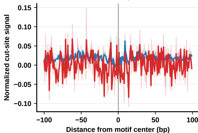
RORC (MA1151.2) T-cell subset-associated regulator, n=5,247 sites
