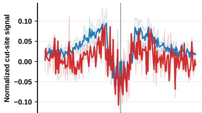
BACH2 (MA1101.3) B/GM12878-biased shared regulator, n=6,500 sites
