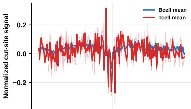
PAX5 (MA0014.4) B-cell lineage regulator, n=3,174 sites
