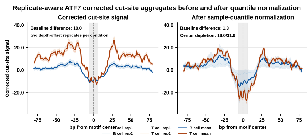
Figure 2. Effect of sample-level quantile normalization on replicate-aware corrected cut-site aggregate profiles. ATACCorrect-corrected B-cell and T-cell matrices were aggregated around ATF7-associated sites and converted into two deterministic depth-offset replicate profiles per condition. Condition means are shown with light replicate-variation ribbons. The raw panel shows a large condition-level baseline offset, whereas sample-level quantile normalization reduces this offset while retaining the central cut-site depletion pattern expected of a footprint. Generated by paper/scripts/plot_normalization_effect.py .
