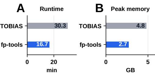
Figure 5. Single-machine runtime and memory check. (A) Runtime and (B) peak memory are summarized for one local analysis run comparing TOBIAS and fp-tools on the same analysis bundle. These measurements are included as an engineering check, not as an exhaustive cross-tool benchmark.
