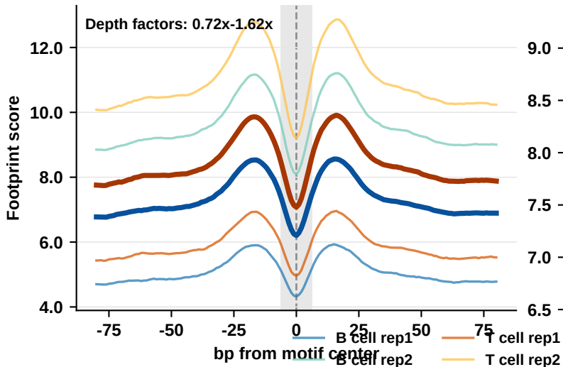
Raw replicate profiles
