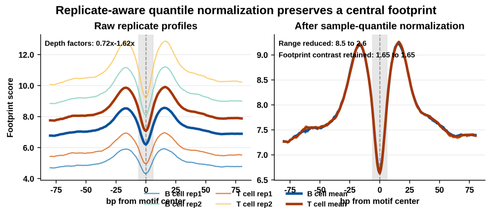
Figure 2. Effect of sample-level quantile normalization on replicate footprint profiles. A controlled two-condition, four-replicate simulation was generated with known replicate-specific depth factors and a central protected footprint. Thin colored lines show individual replicates and thick lines show condition means. The raw panel shows depth-driven amplitude differences, whereas sample-level quantile normalization aligns replicate scales while retaining the central footprint contrast. Generated by paper/scripts/plot_normalization_effect.py .
