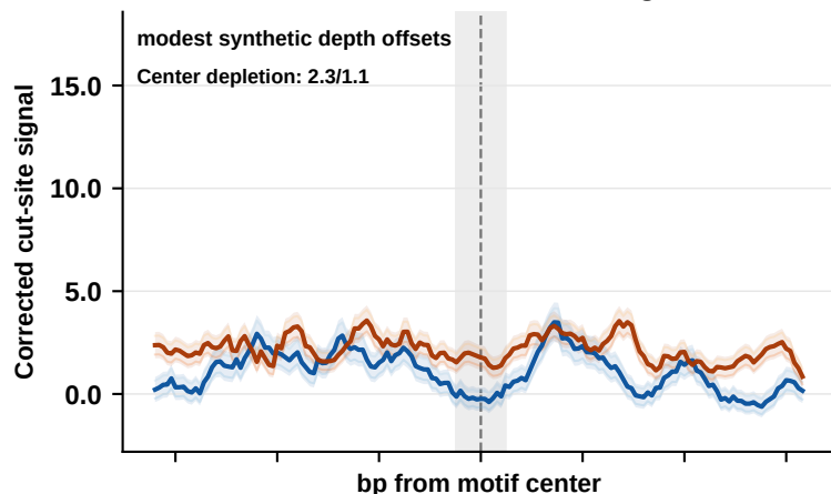
ETS1: corrected cut-site signal
