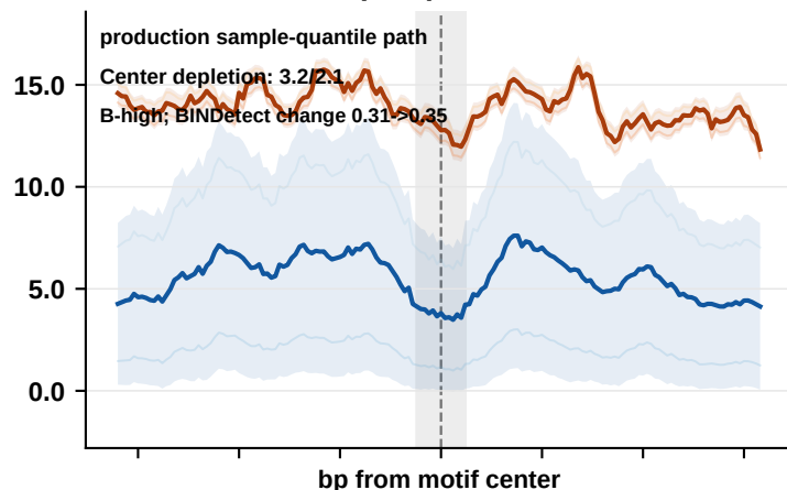
ETS1: after sample-quantile normalization
