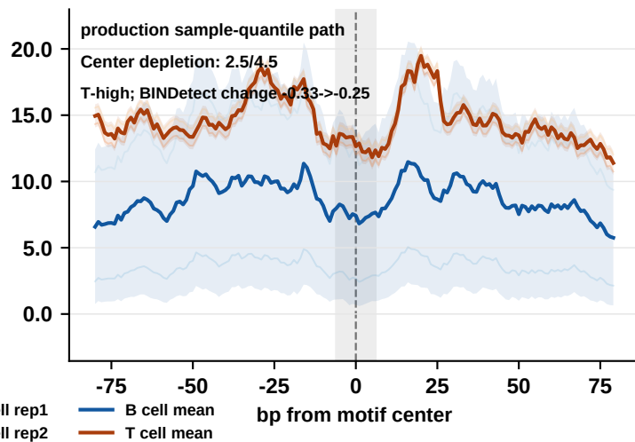
ETS1: after sample-quantile normalization
