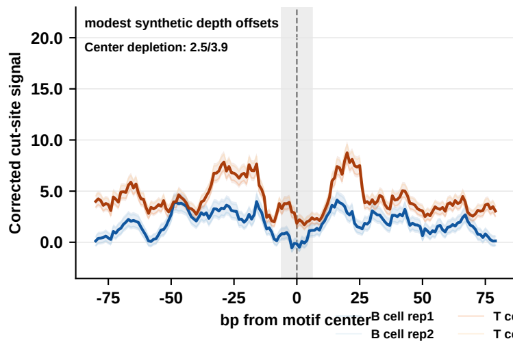
ETS1: corrected cut-site signal
