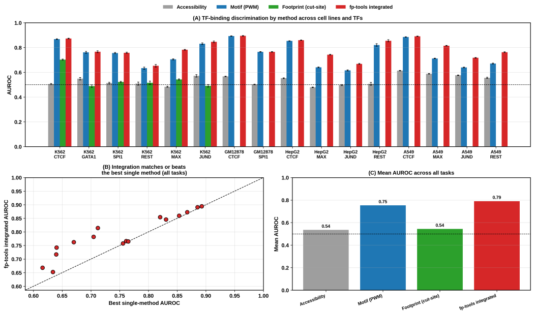
Figure 3. Genome-wide, chromosome-held-out multi-method benchmark across four ENCODE cell lines and 16 cell-TF tasks. Panel A compares per-task AUROC (with bootstrap 95% CIs) for raw accessibility, motif-only scoring, cut-site footprint scoring where available, and the integrated fp-tools model. Panel B compares the integrated model with the best single-method score for each task (points on or above the diagonal mean integration matches or beats the best single method). Panel C summarizes mean AUROC by method. Generated by paper/scripts/plot_method_comparison_multi.py .
