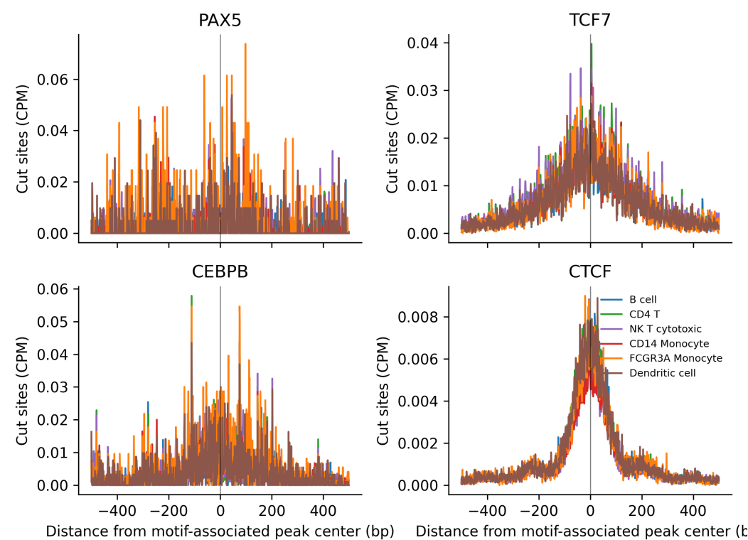
Figure 2. Real 10x PBMC pseudobulk TF aggregate profiles. Single-cell ATAC fragments from the public 10x PBMC Multiome dataset were grouped by broad immune-cell labels derived from official 10x gene-expression graph clusters, converted to CPM-normalized cut-site bigWigs, and aggregated around 10x motif-associated peak centers for PAX5, TCF7/TCF7L2, CEBPB, and CTCF. The figure demonstrates that fp-tools-pseudobulk produces group-level signal tracks that can be visualized by the same aggregate-profile workflow used for bulk ATAC data. Generated by paper/scripts/plot_pseudobulk_tf_aggregates.py .
