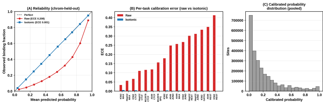
Figure 4. Calibration of the integrated fp-tools probabilities, pooled over all 16 genome-wide tasks under chromosome-held-out evaluation. (A) Reliability diagram: raw class-balanced probabilities are over-confident (red, ECE 0.21), while leak-free isotonic recalibration lands on the diagonal (blue, ECE 0.001). (B) Per-task ECE before and after recalibration. (C) Distribution of calibrated probabilities. Generated by paper/scripts/plot_calibration_panel.py .
