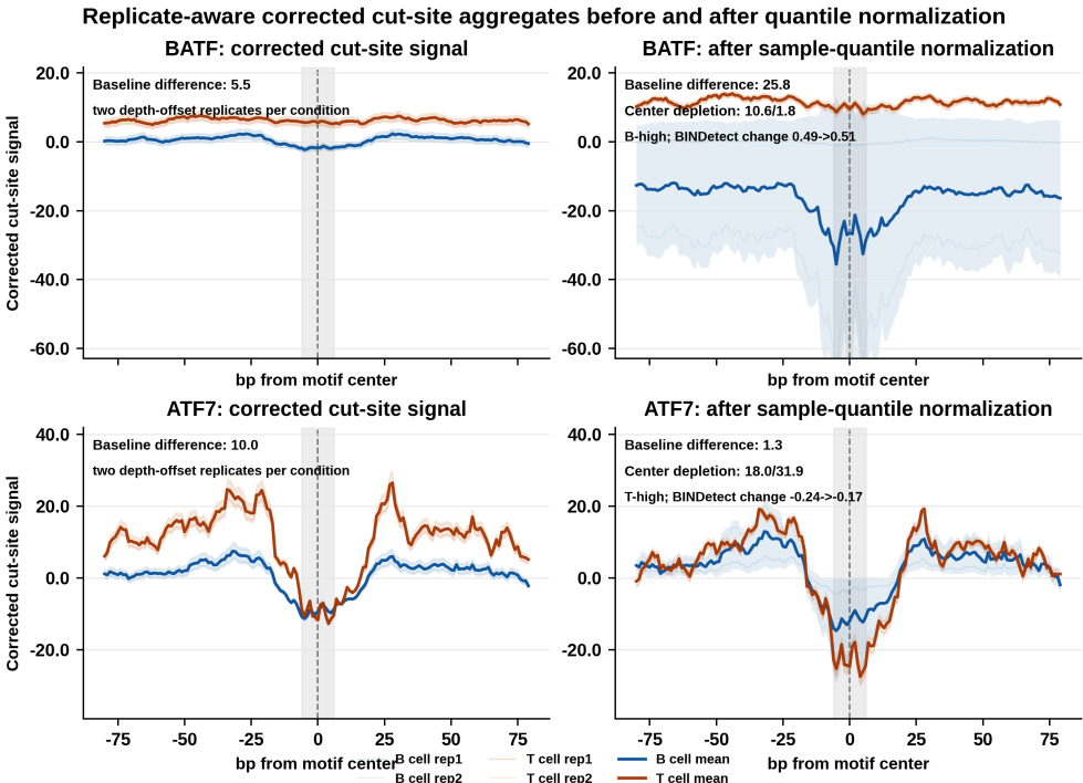
Figure 2. Effect of sample-level quantile normalization on replicate-aware corrected cut-site aggregate profiles. ATACorrect-corrected B-cell and T-cell matrices were aggregated around BATF-associated sites (a normalized B-cell-deeper example) and ATF7-associated sites (a normalized T-cell-deeper example), then converted into two deterministic depth-offset replicate profiles per condition. Condition means are shown with light replicate-variation ribbons. The right column uses the same shared quantile-normalization fit used by replicate-aware detect-tf-binding, plotted on corrected cut-site signal without display-time nonnegative clipping so central depletion remains visible; a lower center relative to the local flanks indicates stronger TF protection. Generated by paper/scripts/plot_normalization_effect.py .
