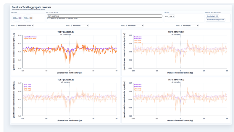
Figure 2. Usability-oriented fp-tools interfaces. (A) Browser GUI for configuring footprinting workflows and saving runnable YAML configurations. (B) Self-contained differential-footprint HTML report from the Buenrostro B-cell versus T-cell replicate comparison, combining differential evidence, selected motif metadata, motif logo display, and aggregate footprint profiles. (C) Aggregate-batch HTML report generated from the same embedded aggregate payload, allowing multi-sample and multi-TF aggregate review with searchable motif selection, group color controls, configurable panel layouts, and editable SVG export.
