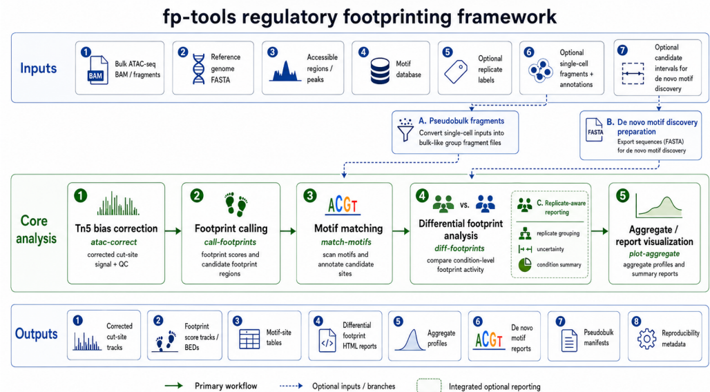
Figure 1. Generic fp-tools regulatory-footprinting framework. Bulk ATAC-seq inputs enter an integrated core for Tn5 bias correction, footprint calling, motif matching, differential footprint analysis, and aggregate visualization. Integrated branches support single-cell pseudobulk fragment generation, de novo motif-discovery preparation from candidate intervals, and replicate-aware reporting within differential comparisons. Outputs include corrected cut-site tracks, footprint score tracks or candidate BEDs, motif-site tables, differential-footprint HTML reports, aggregate profiles, pseudobulk manifests, de novo motif reports, and reproducibility metadata.
