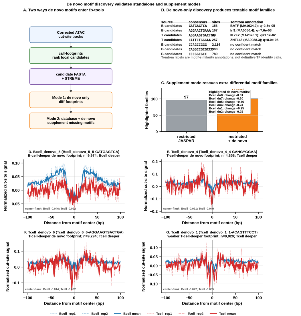
Figure 4. De novo motif discovery used as de novo-only analysis and as a supplement to known-motif analysis. Candidate footprints from the Buenrostro B-cell versus T-cell replicate comparison were exported to FASTA and analyzed with STREME in both contrast directions. The de novo-only branch yields candidate-derived motif families, with representative footprint-like aggregate profiles selected by negative center-versus-flank signal. The supplement branch appends the discovered motifs to a known database before diff-footprints; in the restricted-database sensitivity test, adding 16 candidate-derived motifs increased the highlighted motif-family count from 97 to 101, including 6 de novo-derived highlighted motifs. Tomtom labels indicate motif similarity to database entries. Thin aggregate lines show individual biological replicates and thick lines show condition means.
