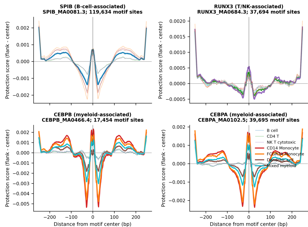
Figure 9. Motif-centered 10x PBMC pseudobulk protection-score aggregate profiles. Single-cell ATAC fragments from the public 10x PBMC Multiome dataset were grouped by broad immune-cell labels derived from official 10x gene-expression graph clusters, converted to CPM-normalized cut-site bigWigs, and aggregated around exact JASPAR2026 motif centers scanned inside 10x ATAC peaks. The plotted score is a flank-minus-center protection summary computed from the pseudobulk cut-site profile, so higher values indicate stronger local center depletion relative to the nearby flanks. SPIB, RUNX3, CEBPB, and CEBPA were selected by the predeclared lineage screen as B-cell-, T/NK-cell-, and myeloid-associated examples. Thin lines show all retained pseudobulk groups; thicker lines mark the expected pseudobulk groups for each lineage-associated TF. The source screen and natural motif-hit counts are reported in figures/supp_pseudobulk_tf_screen.tsv . The figure demonstrates that the pseudobulk fragment workflow produces group-level signal tracks compatible with motif-centered aggregate visualization.
