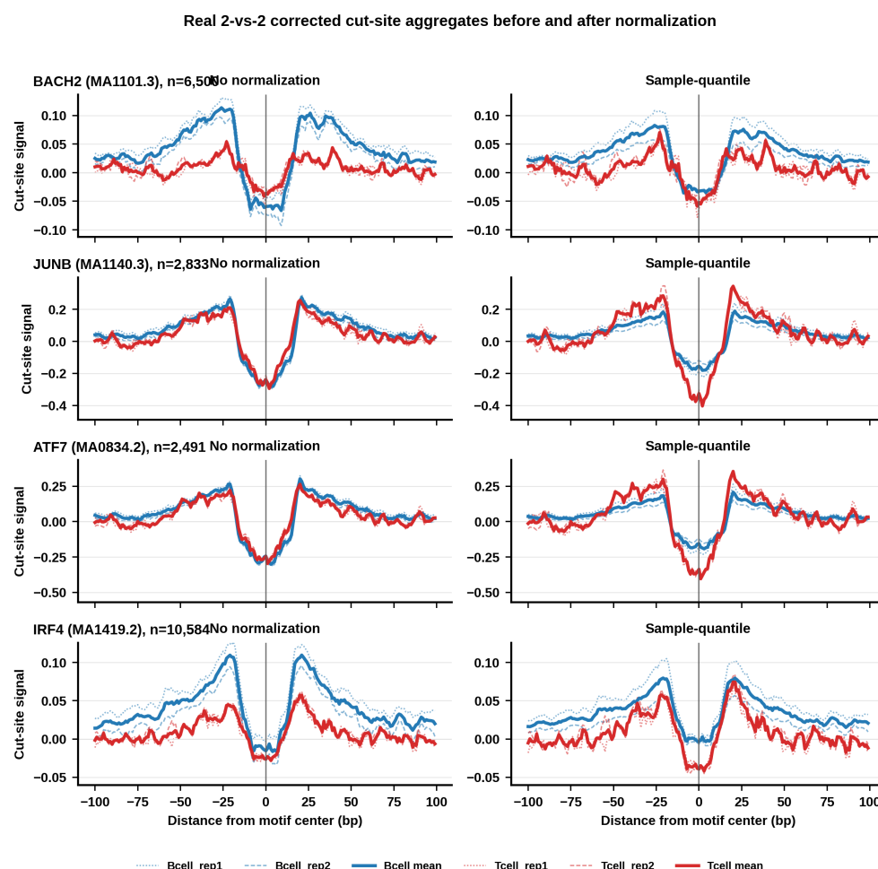
Figure 6. Effect of sample-level quantile normalization on real 2-vs-2 corrected cut-site aggregate profiles. BACH2, JUNB, ATF7, and IRF4 aggregates were extracted from the no-normalization and sample-quantile diff-footprints HTML reports for the Buenrostro B-cell versus T-cell replicate comparison. Thin lines show individual biological replicates, thick lines show condition means, and a lower center relative to the local flanks indicates stronger TF protection.
