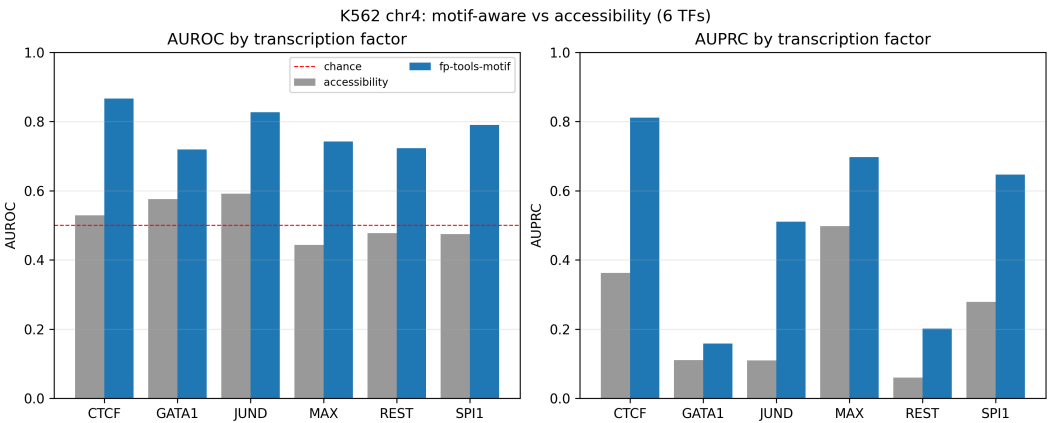
Figure 1. AUROC and AUPRC for a raw accessibility baseline (grey) versus motif-aware scoring (blue) across six K562 transcription factors on ENCODE ATAC-seq peaks (chromosome 4) labeled by matched ChIP-seq overlap. Motif-aware scoring exceeds the accessibility baseline—and the chance line (red)—for every factor. Generated by paper/scripts/plot_method_comparison.py .
