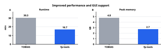
Figure 5. Single-machine runtime and memory check. (A) Runtime and (B) peak memory are summarized for one local analysis run comparing TOBIAS and fp-tools on the same analysis bundle. These measurements are included as an engineering check, not as an exhaustive cross-tool benchmark.
