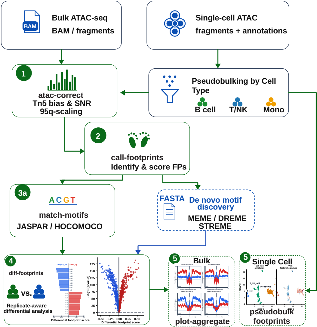
Figure 1. Overview of the fp-tools ATAC-seq footprinting platform. Bulk ATAC-seq BAM/fragments and single-cell ATAC fragments with annotations enter a shared command-oriented workflow. The workflow supports Tn5 bias correction, footprint calling, motif matching against curated databases, de novo motif discovery, replicate-aware differential footprint analysis, aggregate footprint visualization, and pseudobulk single-cell footprint analysis.
