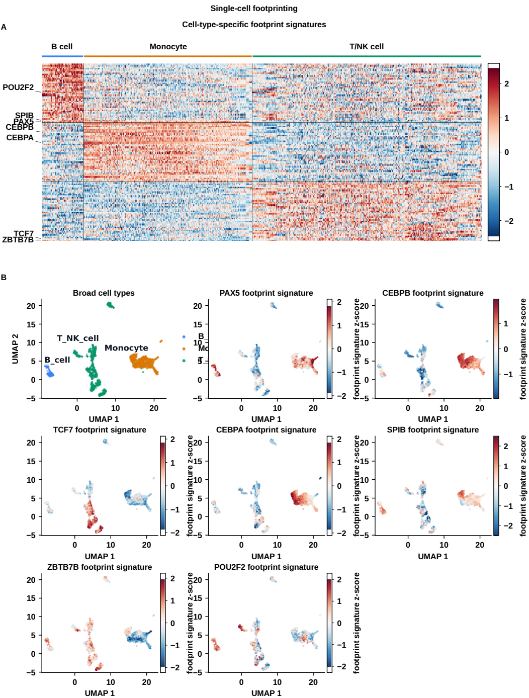
Figure 4. Single-cell footprinting summary in public PBMC5k single-cell ATAC data. (A) KNN-smoothed per-cell footprint-signature heatmap for selected marker TFs and top cell-type-specific motif signatures across B cells, monocytes, and T/NK cells. (B) UMAP projections show broad cell-type annotations and representative marker footprint-signature z-scores. Positive values indicate the marker-oriented footprint-signature direction after per-TF standardization; formal corrected footprint inference is performed at the pseudobulk level.
