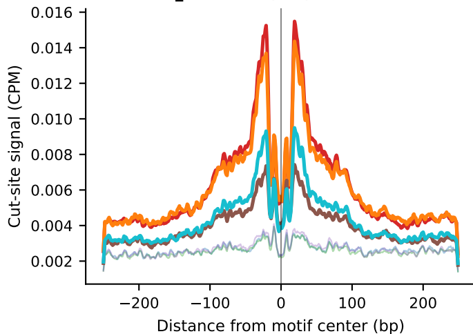
CEBPB (myeloid-associated) CEBPB_MA0466.4; 17,454 motif sites
