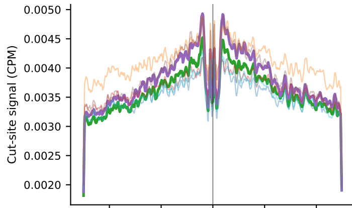
CEBPA (myeloid-associated) CEBPA_MA0102.5; 39,695 motif sites
