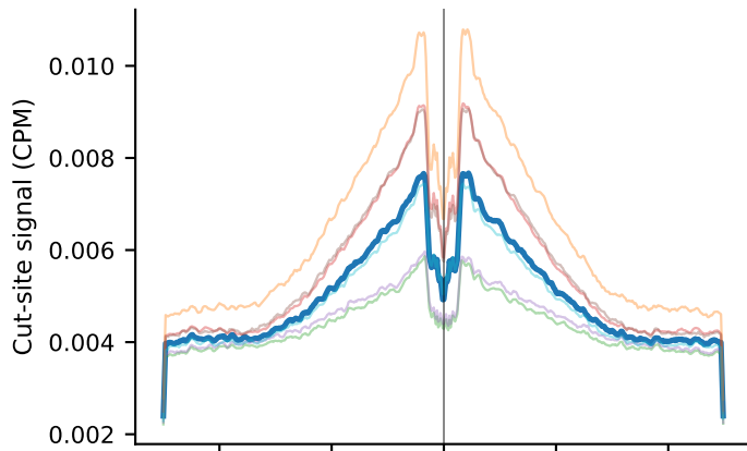
CEBPB (myeloid-associated) CEBPB_MA0466.4; 17,454 motif sites
