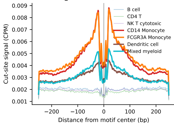
CEBPA (myeloid-associated) CEBPA_MA0102.5; 39,695 motif sites
