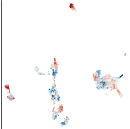
STAT3 (STAT3_MA0144.3)
