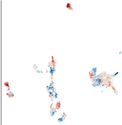
Stat5b (Stat5b_MA1625.2)
