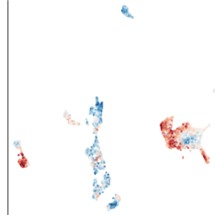
CEBPD (CEBPD_MA0836.3)
