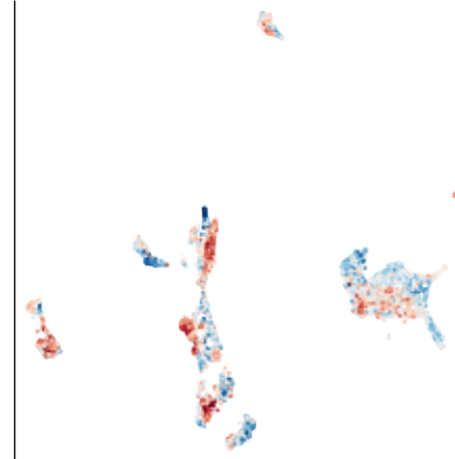
MSANTD3 (MSANTD3_MA1523.2)
