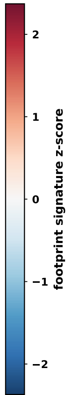
MSANTD3 (MSANTD3_MA1523.2)
