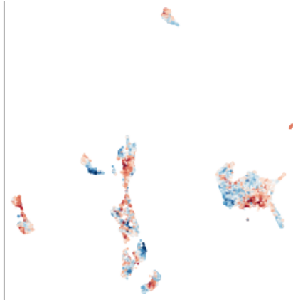
Hic1 (Hic1_MA0739.2)
