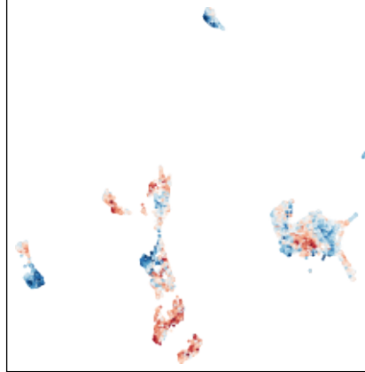
GCM1 (GCM1_MA0646.2)
