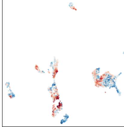
THRA (THRA_MA1969.2)
