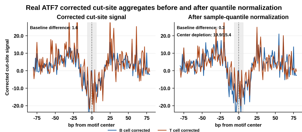
Figure 2. Effect of sample-level quantile normalization on real corrected cut-site aggregate profiles. ATACCorrect-corrected B-cell and T-cell tracks were aggregated around ATF7-associated sites. Solid colored lines show the corrected profiles for each condition. The raw panel shows a condition-level baseline offset, whereas sample-level quantile normalization reduces this offset while retaining the central cut-site depletion pattern expected of a footprint. Generated by paper/scripts/plot_normalization_effect.py .
