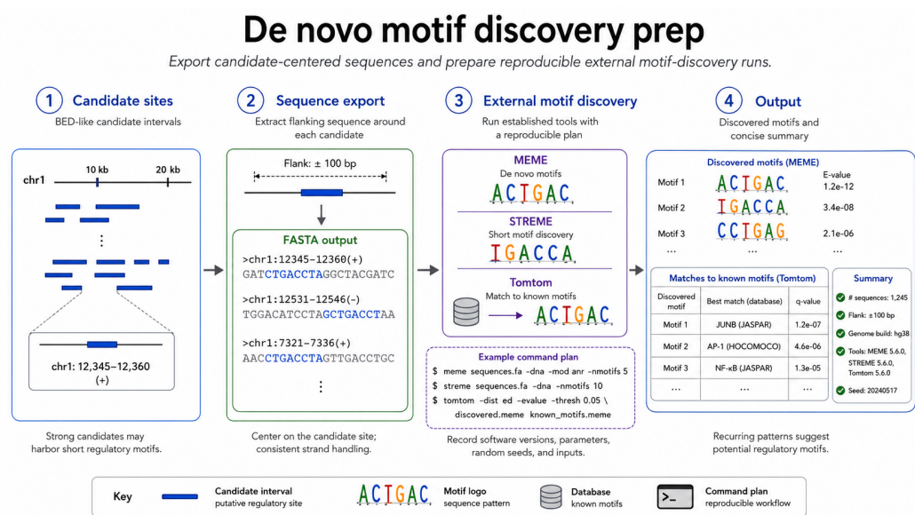
Figure 2. De novo motif-discovery preparation workflow. Candidate-centered sequences are exported from BED-like intervals, external MEME/STREME and Tomtom runs are captured as reproducible command plans, and motif summaries are returned as concise tables and reports. This first-version utility prepares reproducible motif-discovery inputs and reports without claiming a new motif-calling algorithm.
