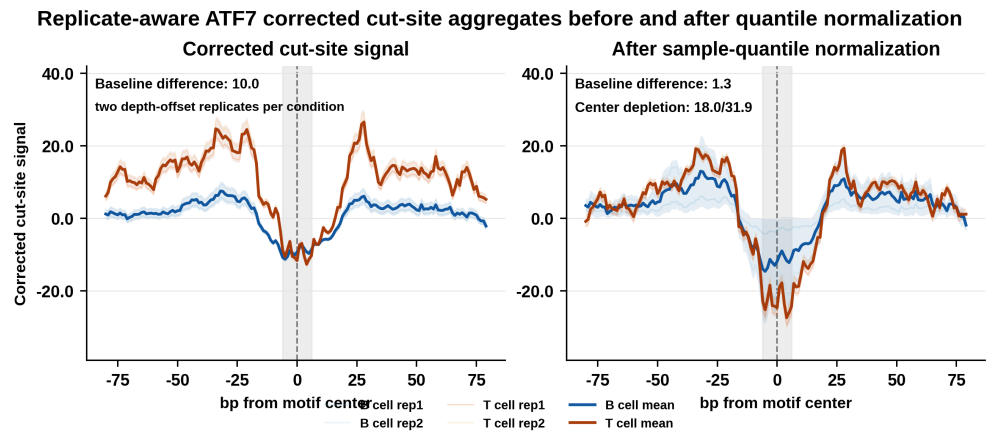
Figure 2. Effect of sample-level quantile normalization on replicate-aware corrected cut-site aggregate profiles. ATACorrect-corrected B-cell and T-cell matrices were aggregated around ATF7-associated sites and converted into two deterministic depth-offset replicate profiles per condition. Condition means are shown with light replicate-variation ribbons. The raw panel shows a large condition-level baseline offset, whereas sample-level quantile normalization reduces this offset while retaining the central cut-site depletion pattern expected of a footprint. Generated by paper/scripts/plot_normalization_effect.py .
