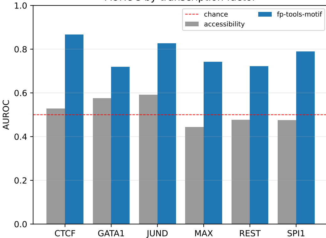
AUROC by transcription factor
