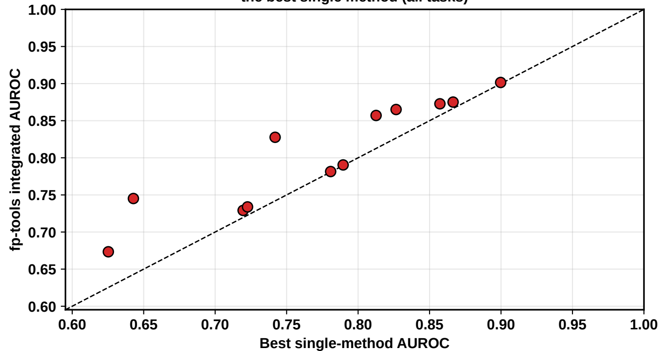
(B) Integration matches or beats the best single method (all tasks)
