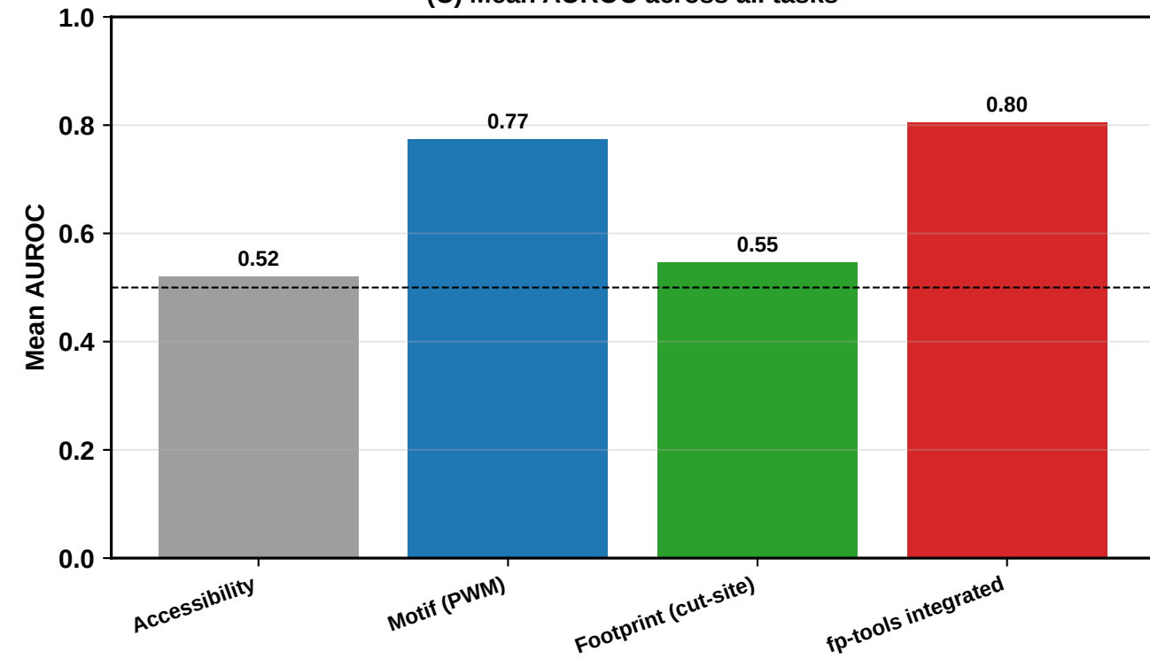
(C) Mean AUROC across all tasks
