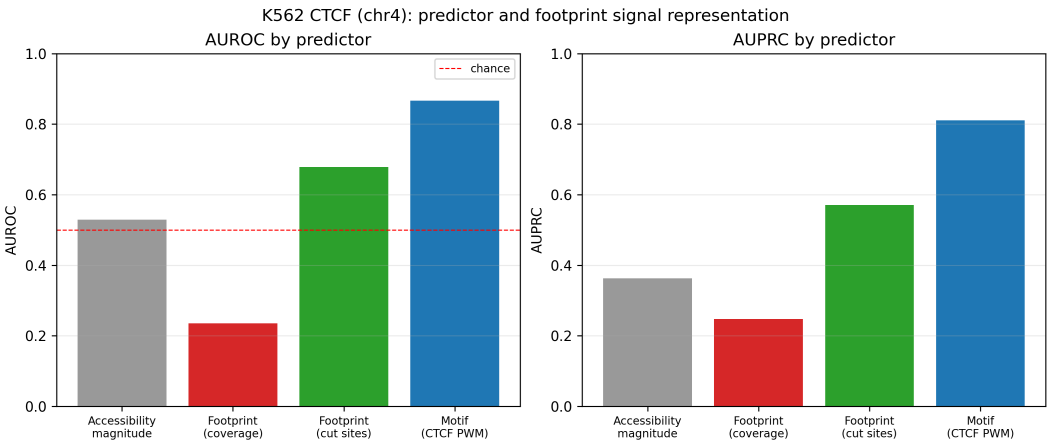
Figure 4. Predictor comparison for K562 CTCF (chromosome 4). A footprint-occupancy score is informative only at Tn5 cut-site resolution (green, AUROC 0.68); the same score on smoothed coverage is inverted and uninformative (red, 0.24). Raw accessibility (grey) is near chance and the CTCF motif (blue) is the single strongest predictor.
