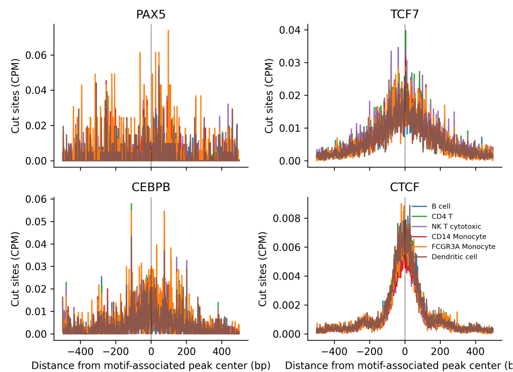
Figure 3. Real 10x PBMC pseudobulk TF aggregate profiles. Single-cell ATAC fragments from the public 10x PBMC Multiome dataset were grouped by broad immune-cell labels derived from official 10x gene-expression graph clusters, converted to CPM-normalized cut-site bigWigs, and aggregated around 10x motif-associated peak centers for PAX5, TCF7/TCF7L2, CEBPB, and CTCF. The figure demonstrates that fp-tools-pseudobulk produces group-level signal tracks that can be visualized by the same aggregate-profile workflow used for bulk ATAC data. Generated by paper/scripts/plot_pseudobulk_tf_aggregates.py .
