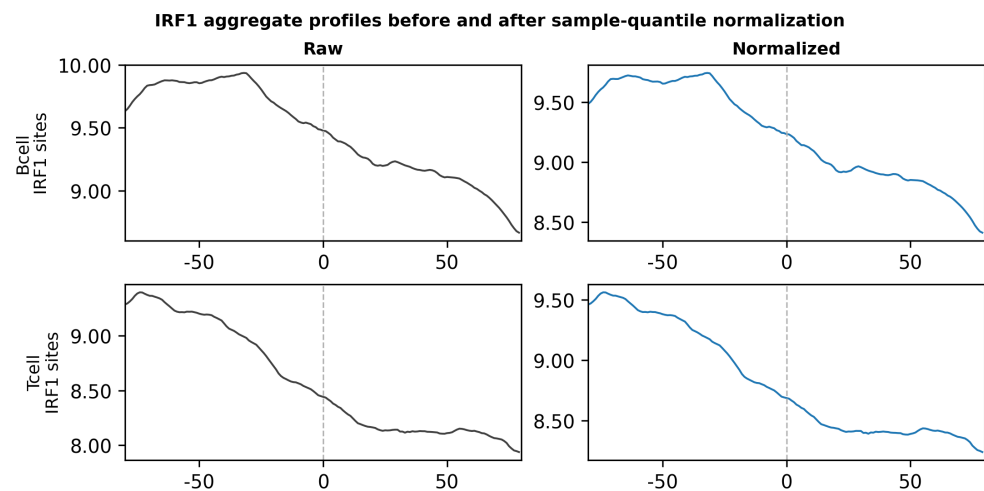
Figure 2. Effect of sample-level quantile normalization on replicate aggregate profiles. IRF1 aggregate profiles were computed from existing B-cell and T-cell footprint tracks after applying controlled replicate-specific scale factors. The raw panels show depth-driven amplitude differences between simulated replicates and conditions, whereas sample-level quantile normalization reduces scale differences while retaining the aggregate footprint profile around IRF1 sites. Generated by paper/scripts/plot_normalization_effect.py .
