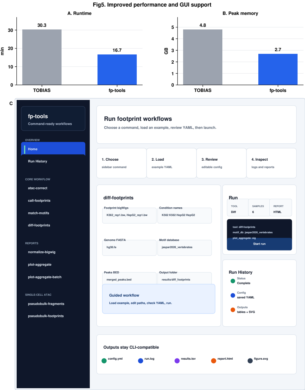
Figure 5. Improved performance and GUI support. (A,B) Representative local engineering comparisons of runtime and peak memory between TOBIAS and fp-tools. (C) The browser GUI provides a command-first interface for configuring inputs, saving reusable configs, running core footprinting steps, and reviewing logs, tables, and SVG-ready outputs while preserving CLI compatibility.
