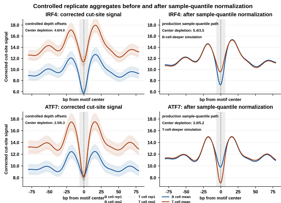
Figure 2. Effect of sample-level quantile normalization on replicate-aware corrected cut-site aggregate profiles. Controlled B-cell and T-cell aggregate profiles were simulated with IRF4 as a B-cell-deeper example and ATF7 as a T-cell-deeper example, then converted into two deterministic, moderately depth-offset replicate profiles per condition. Condition means are shown with light replicate-variation ribbons. The right column uses the same nonnegative-clamped sample-quantile normalization path used by replicate-aware detect-tf-binding and plot-aggregate; raw baseline offsets are reduced and a lower center relative to the local flanks indicates stronger TF protection. Generated by paper/scripts/plot_normalization_effect.py .
