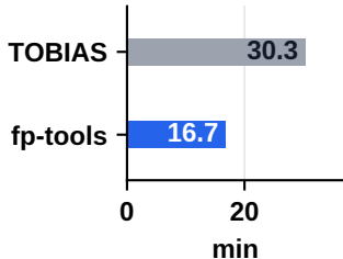
A Runtime
