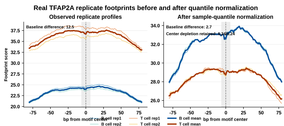
Figure 2. Effect of sample-level quantile normalization on real replicate footprint profiles. Observed B-cell and T-cell replicate footprint tracks were aggregated around TFAP2A-associated sites. Thin colored lines show individual replicates and thick lines show condition means. The raw panel shows a condition-level baseline offset, whereas sample-level quantile normalization reduces this offset while retaining the central depletion pattern expected of a footprint. Generated by paper/scripts/plot_normalization_effect.py .
