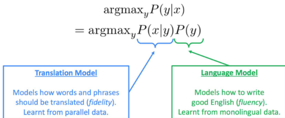
Figure 9: Statistical Machine Translation: разложение задачи перевода на translation model и language model.
