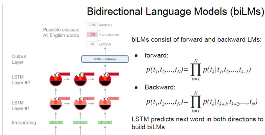
Figure 29: ELMo использует bidirectional language model: forward и backward LSTM.
